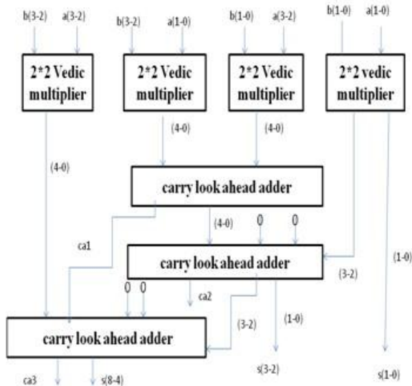
Fig.6. Block diagram for 4-bit Vedic multiplication
