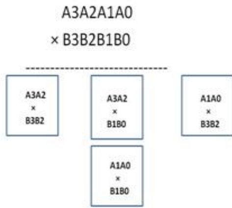
Fig.5. A sample representation of 4-bit Vedic multiplication
