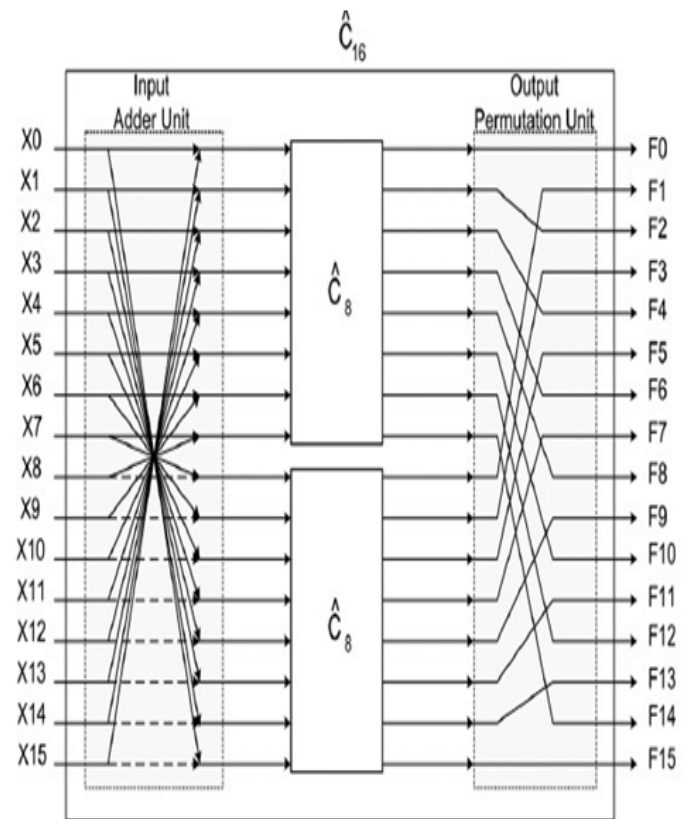
Fig.2. Block diagram of approximation of DCT for n=16
