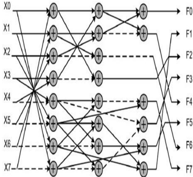
Fig.1. Signal Flow Graph (sfg) of (c8).
